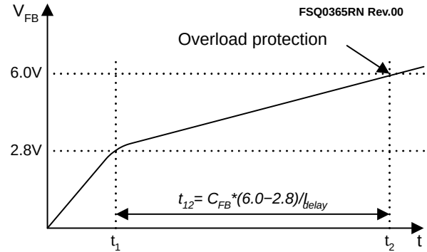
Figure 24. Overload Protection
